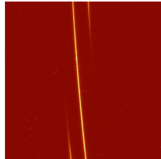
FeI 1650: 60nm (1.616-1.676 \mu\text{m} )
