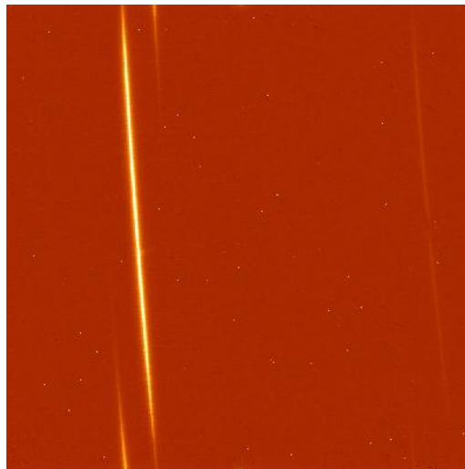
FeI 1252: 25nm (1.239-1.265 \mu\text{m} )
