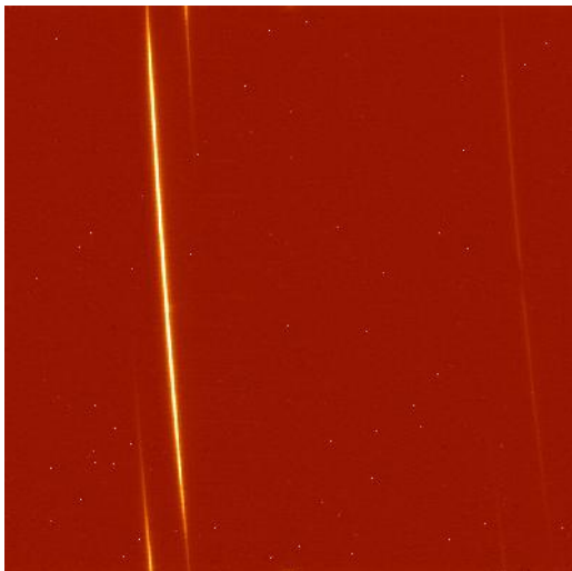
He 1085: 20nm (1.073-1.093 \mu\text{m} )
