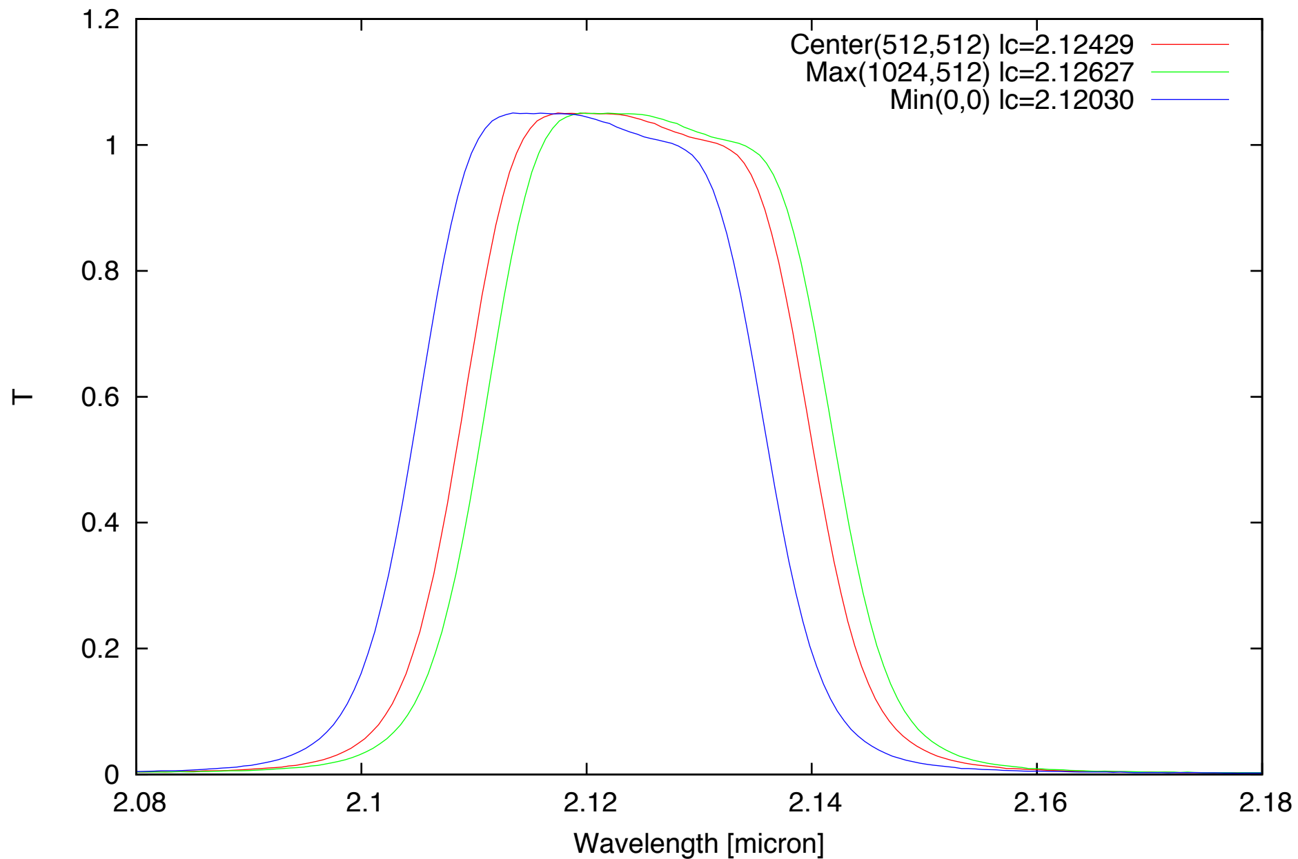
IRCS H2(1-0) filter Width=316A
