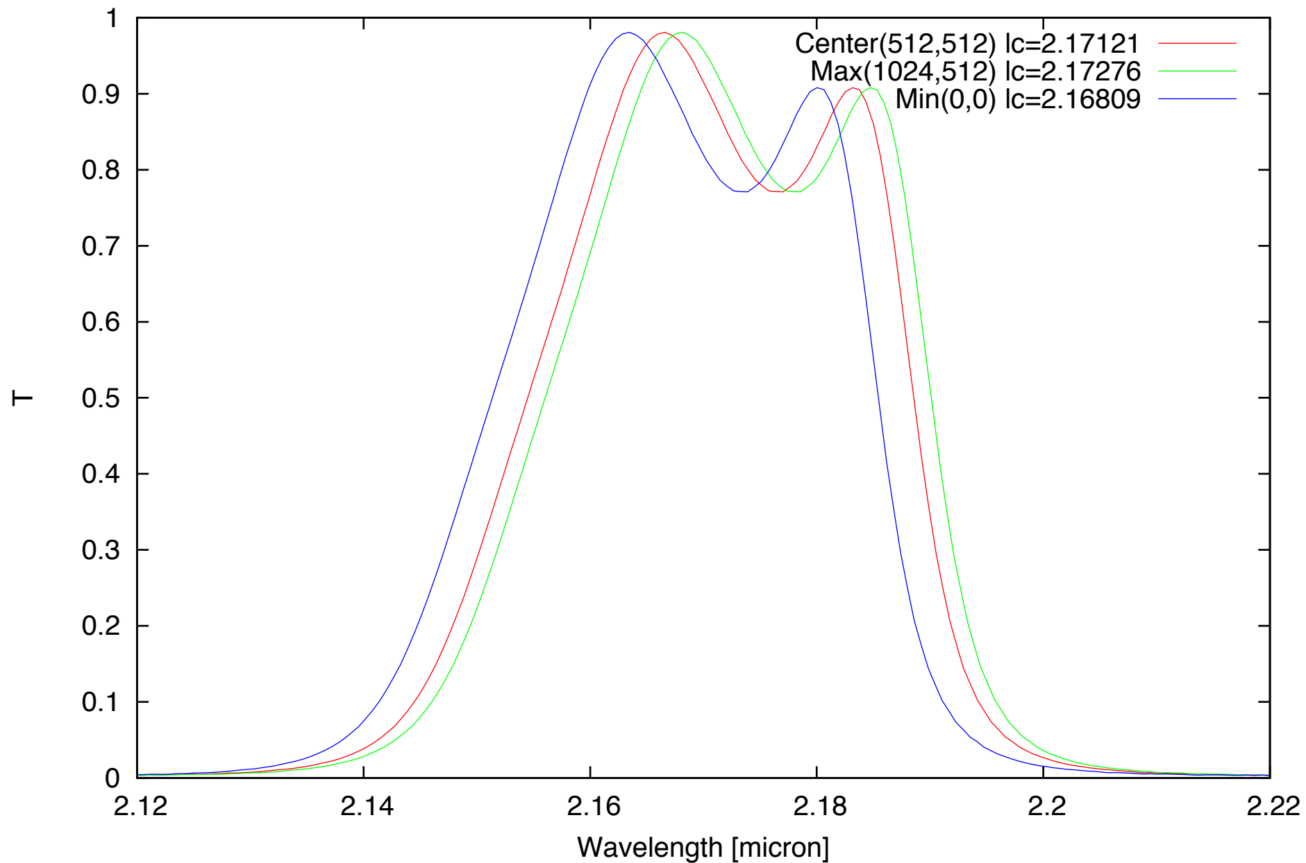
IRCS BrG filter (width=355.5Å)
