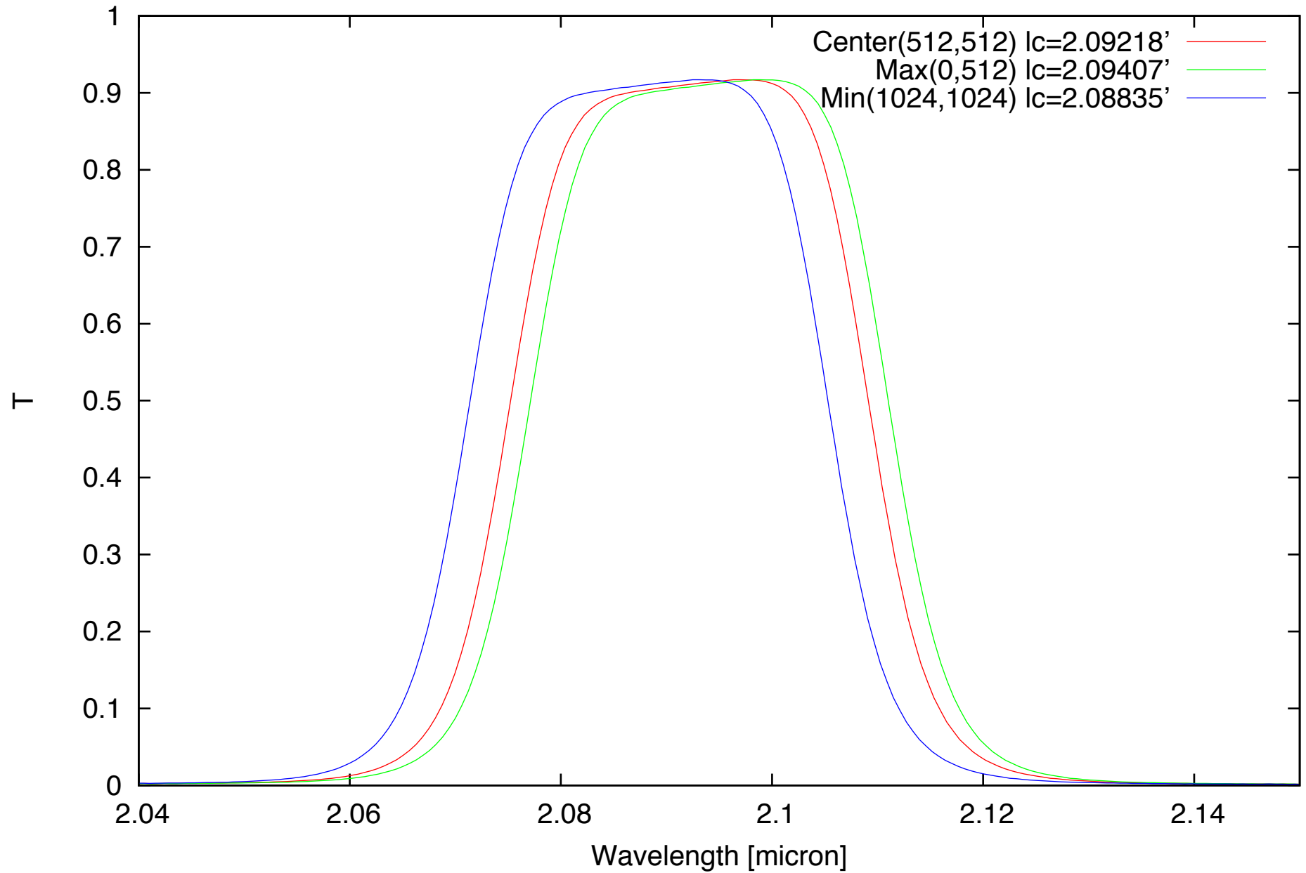
IRCS NB209 filter Width=350A
